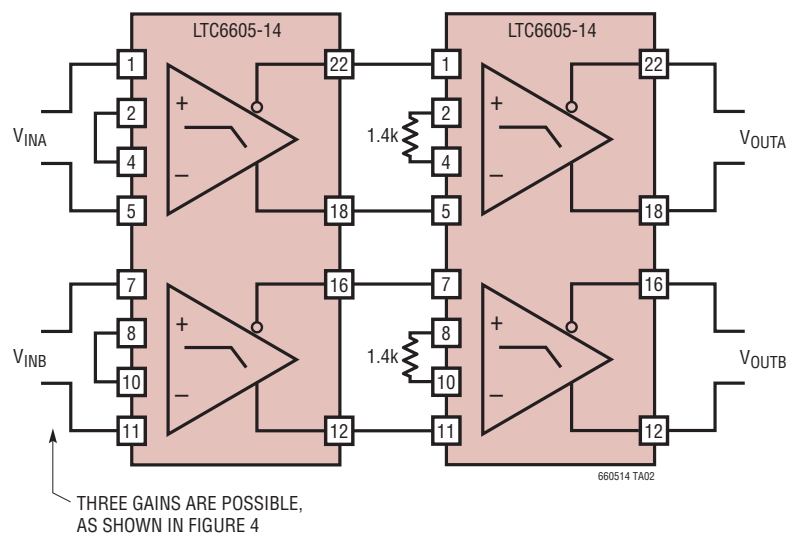
Dual, Matched, 4th Order 14MHz Lowpass Filter
